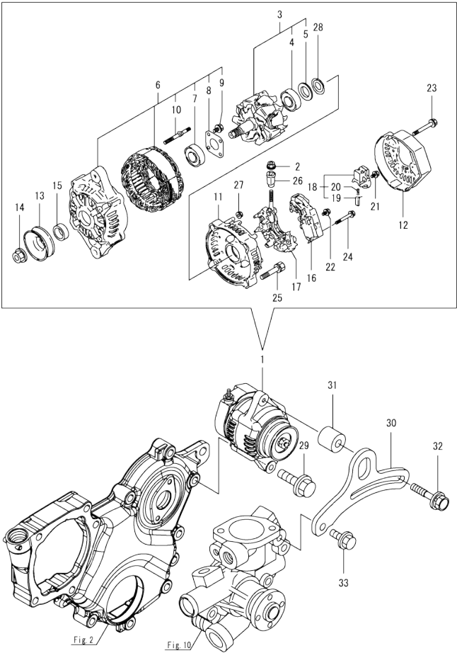
OCD50-M02390 ENGINE Fig.16. GENERATOR
