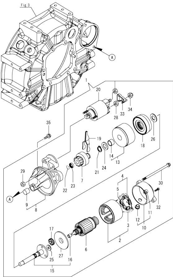
Fig.15. STARTER MOTOR
